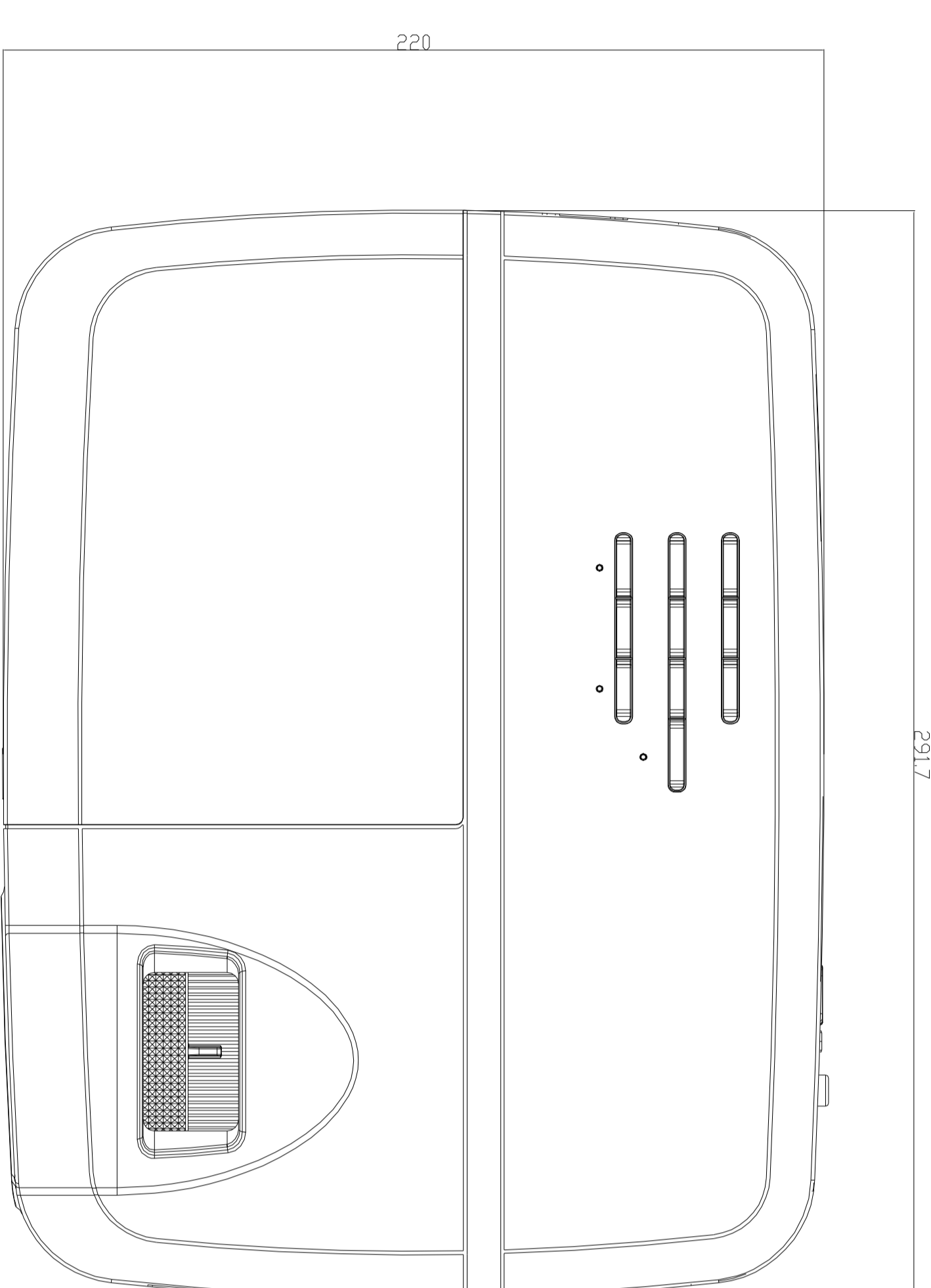
TOP VIEW
